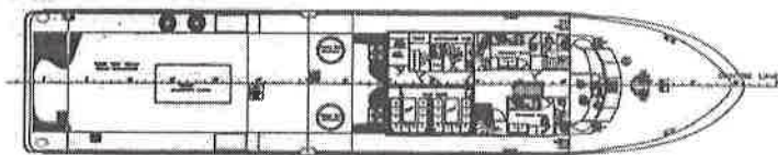
DECK PLAN
